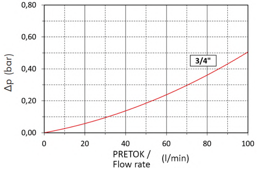
PADEC TLAKA / Pressure drop
